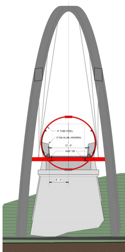
2 SECTION 2 A 100 3/16" = 1'-0"
